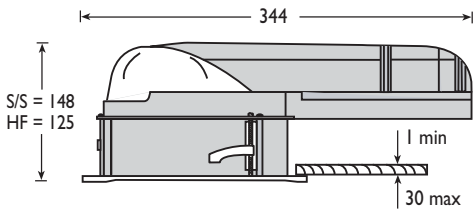
IP65 version
